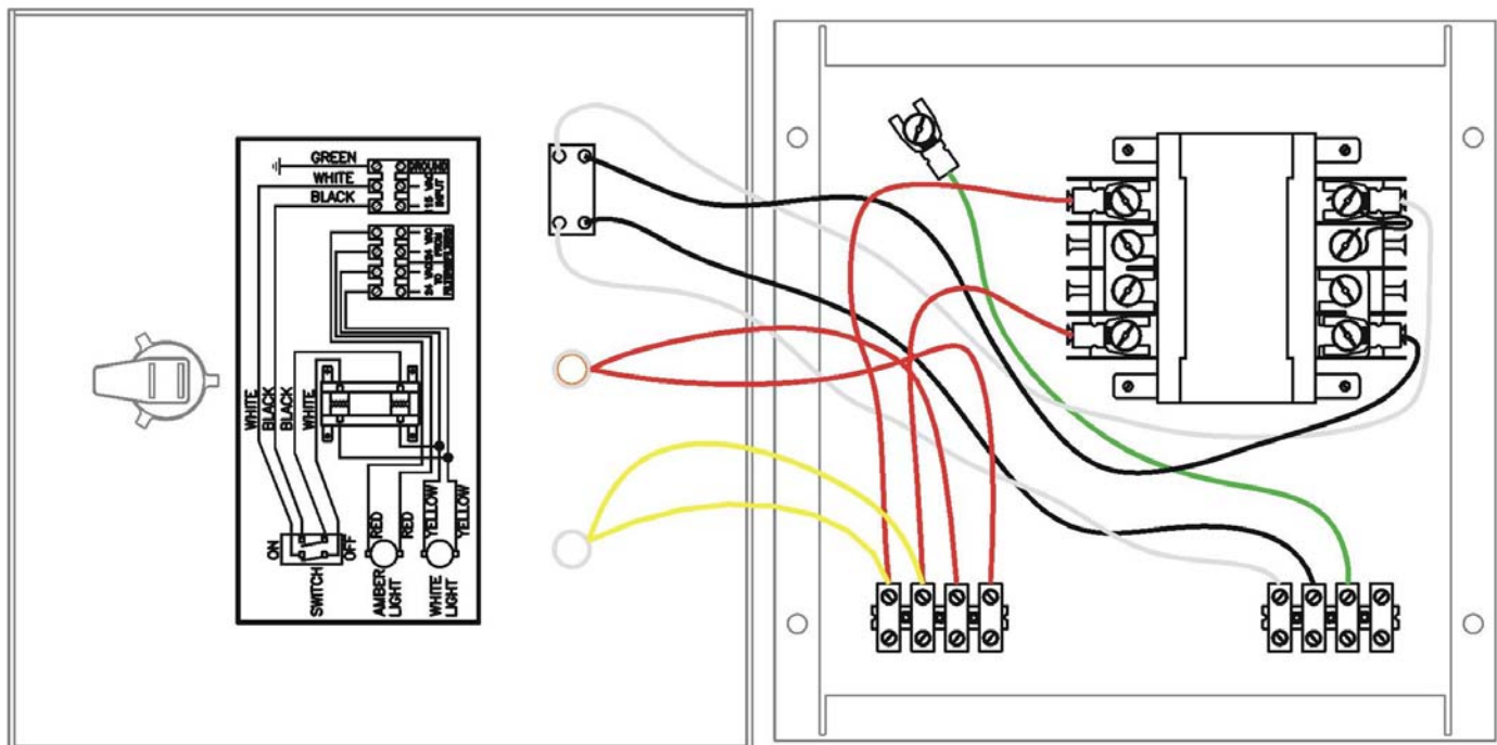
Electrical Circuit
